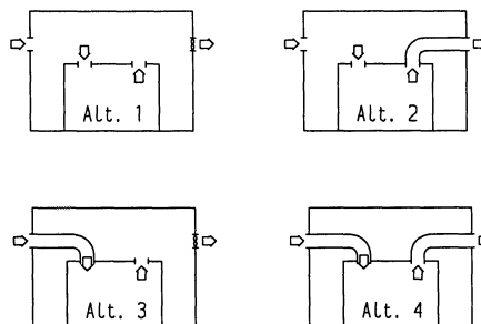
VENTILATION PROPOSALS (1)
