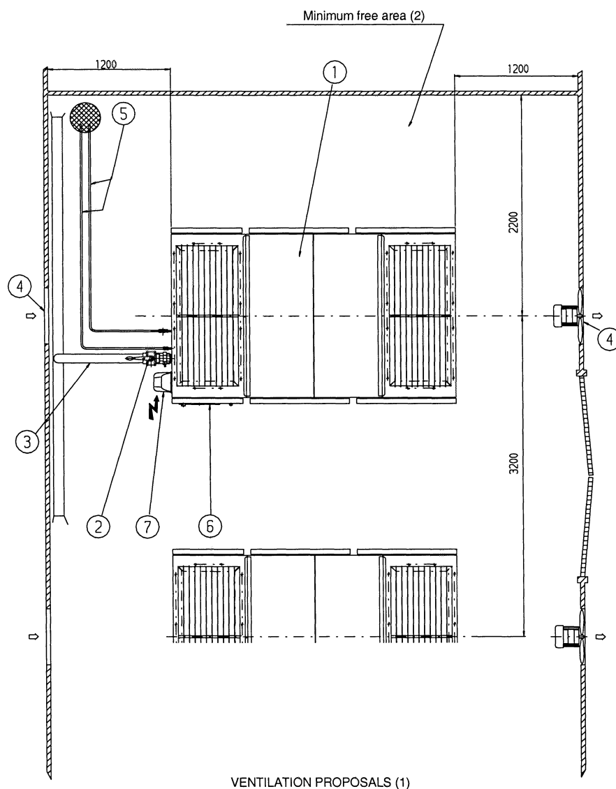
VENTILATION PROPOSALS (1)
