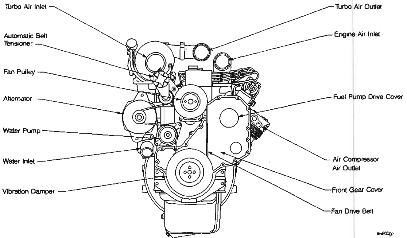
Front View
